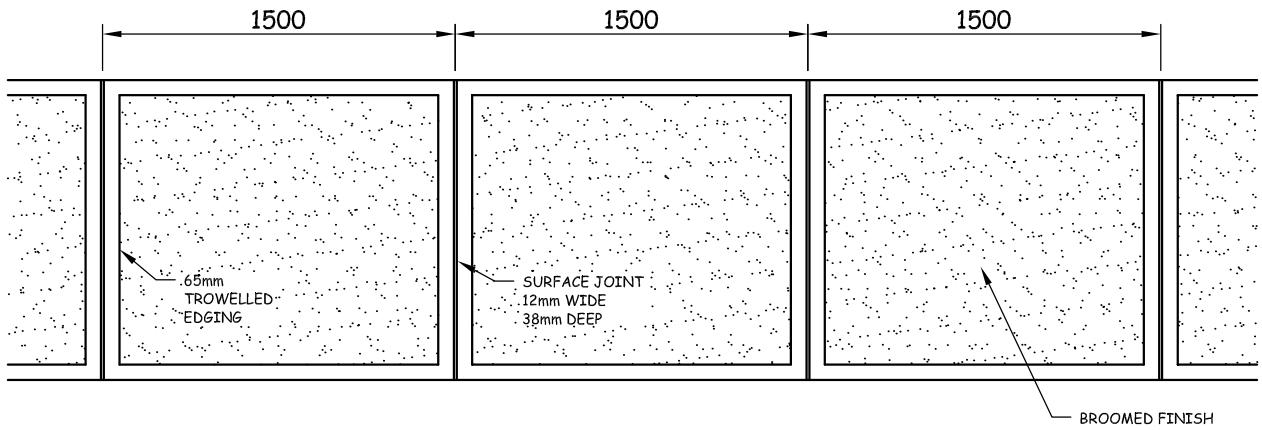
PLAN VIEW
