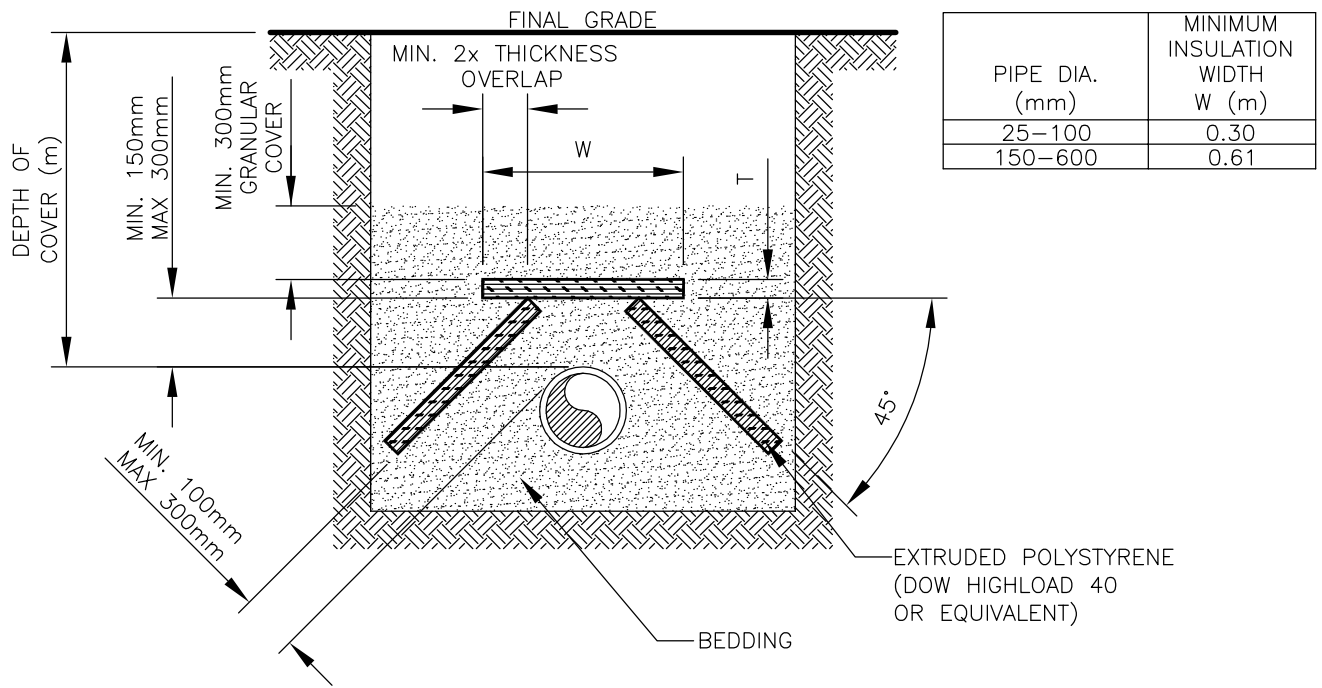
INSULATION DETAIL FOR STANDARD TRENCH EXCAVATION
