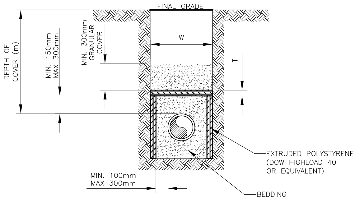
INSULATION DETAIL FOR NARROW TRENCH EXCAVATION
