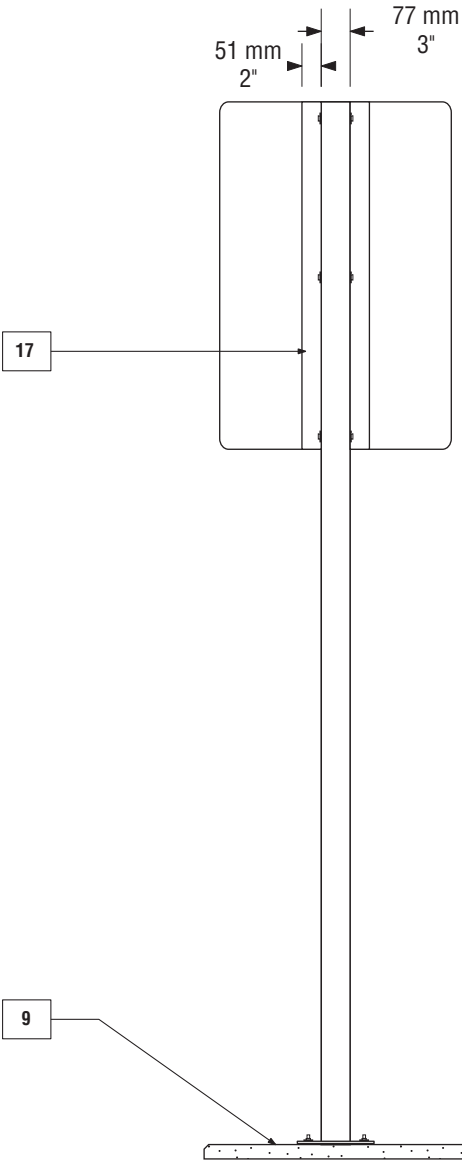
IN-4 Single-post Information Large • Rear View (Typical)
