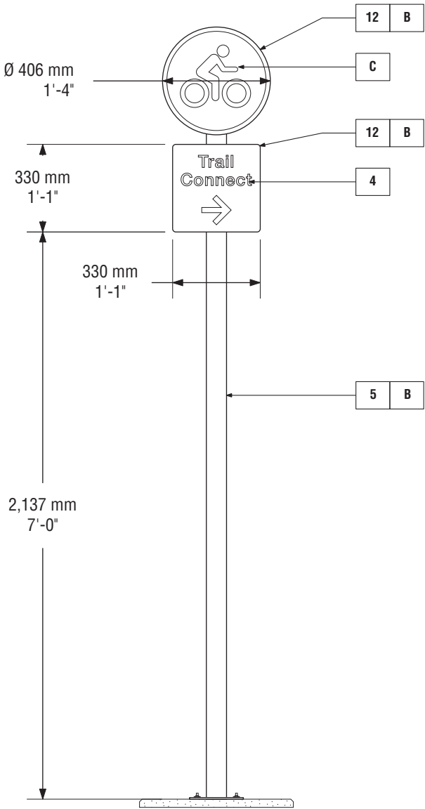
D-2 Trail Connect • Front View (Typical)
