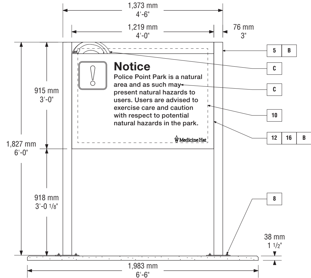
IN-3 Tertiary Information Hub • Front View (Typical)
