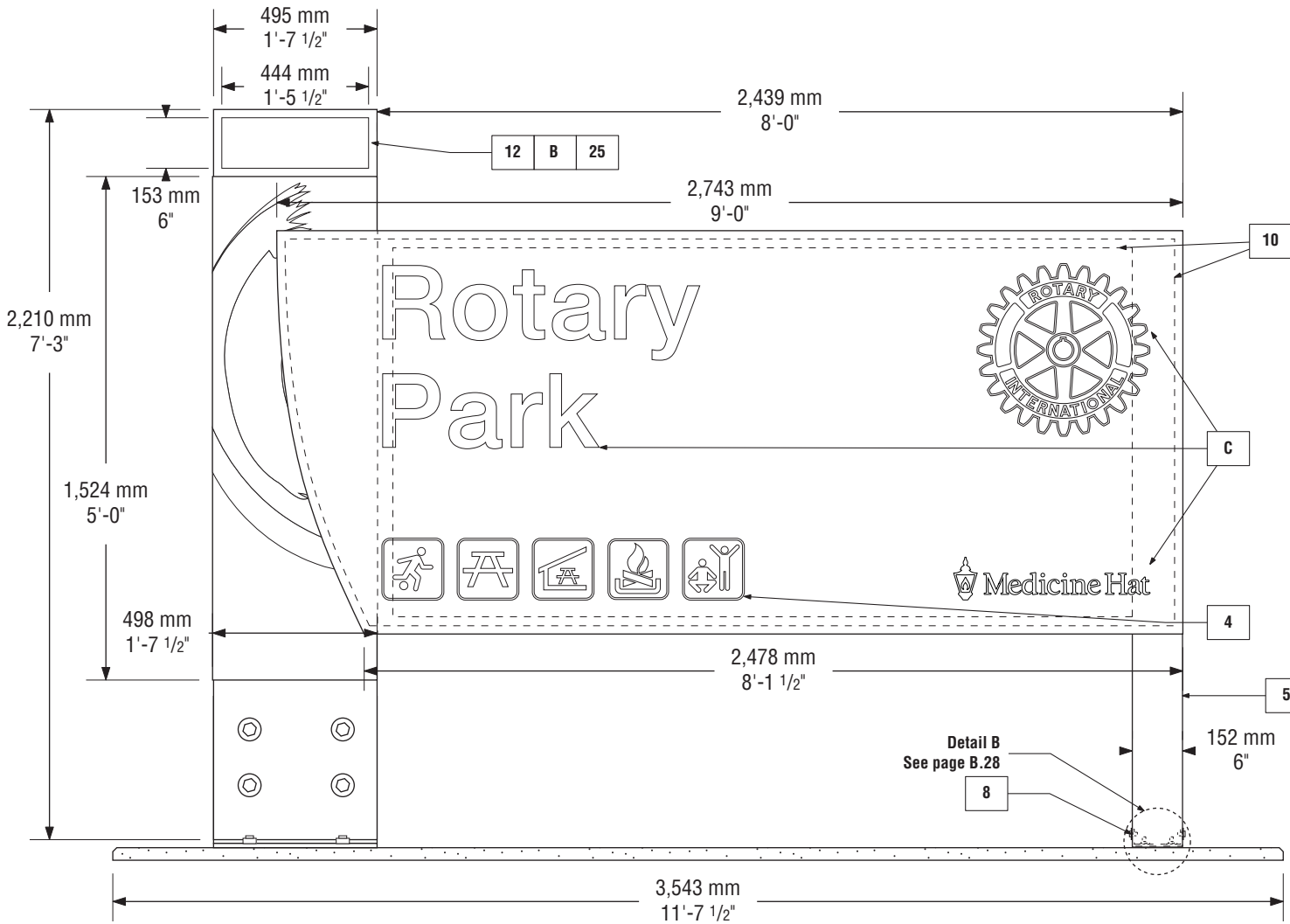
IDP-1 Primary Park Identification • Front View (Typical)
