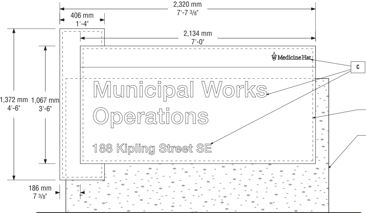
IDF-2 Retrofit Facility ID • Front View (Typical)
