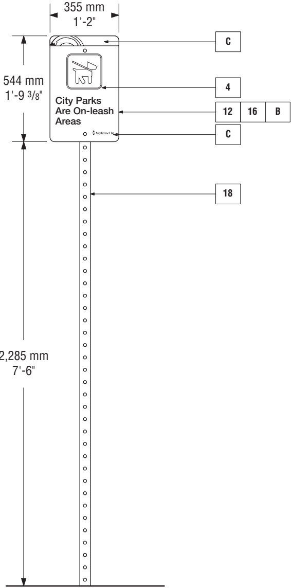
IN-5 Single-post Information Small • Front View (Typical)
