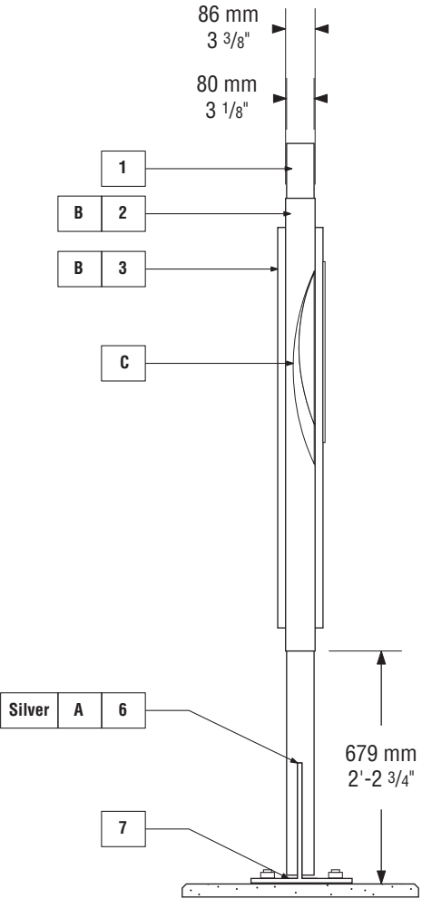
IN-2 Secondary Information Hub • Left View/Right View (Typical)
