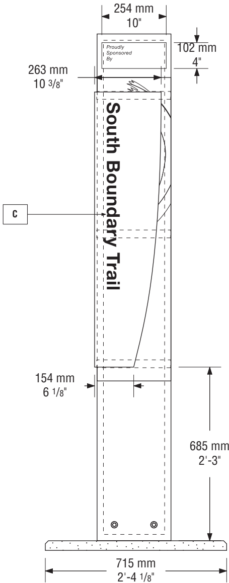
D-1 Trail Marker • Side B (Typical)
