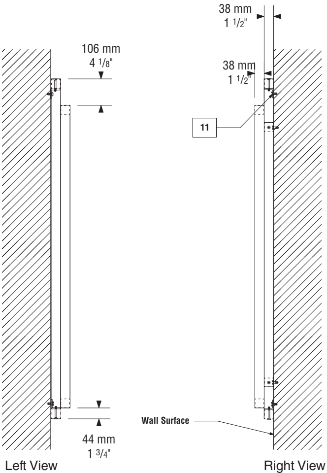
IDF-3 Wall Mounted Facility ID • Left View/Right View (Typical)
