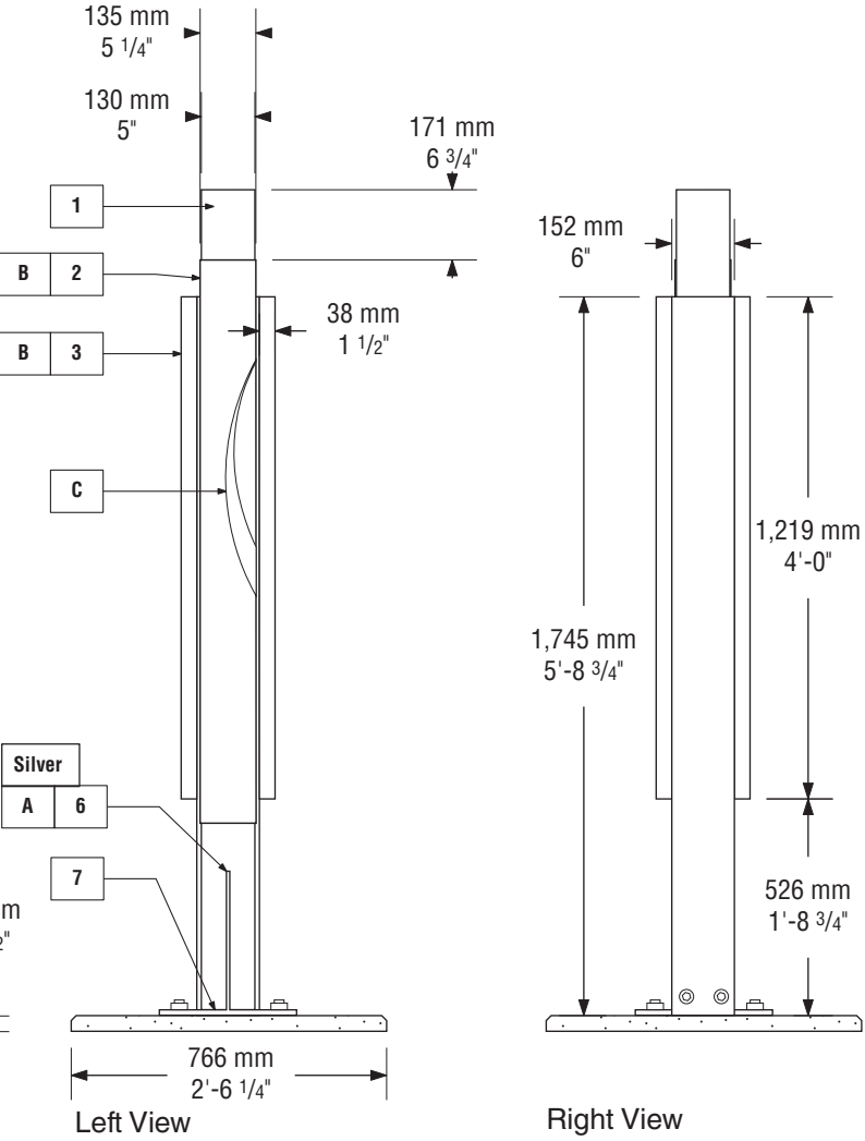
IDP-2 Secondary Park Identification • Left View/Right View (Typical)
