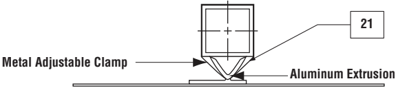
Square Pole Mounting Details • Plan
