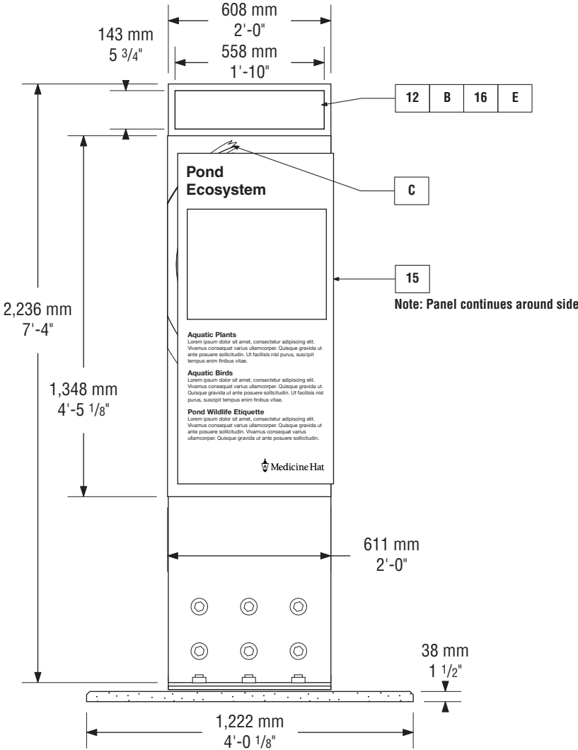
INT-1 Primary Interpretive • Front View (Typical)
