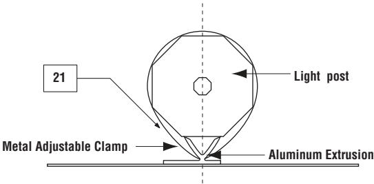
Light Pole Mounting Details • Plan
