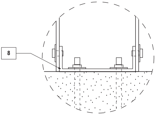
Detail B Scale: NTS Note: Dimensions will vary. TBD by sign supplier.
