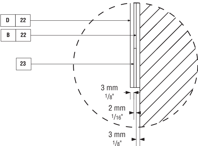
T-1 Temporary Information Small • Detail A
