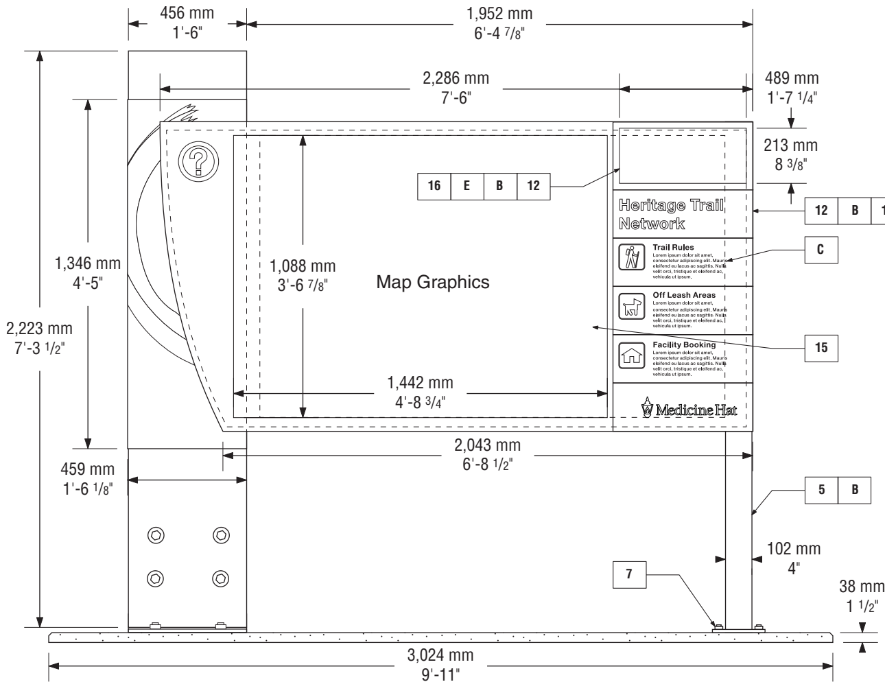
IN-1 Primary Information Hub • Front View (Typical)
