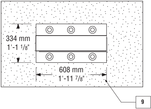
INT-1 Primary Interpretive • Top View (Typical)
