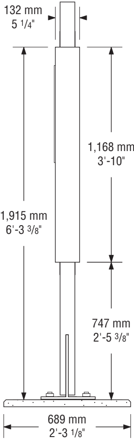
IN-2 Secondary Information Hub • Left View/Right View (Typical)
