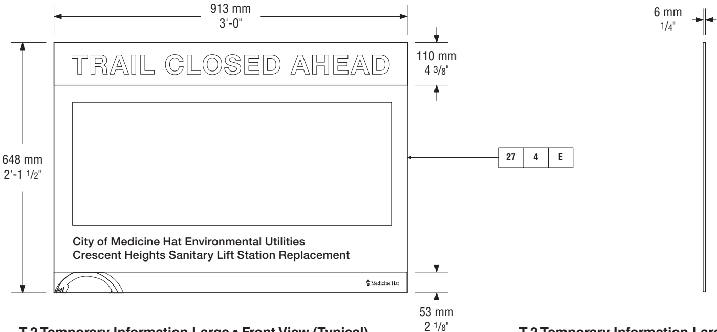
T-2 Temporary Information Large • Front View (Typical)
