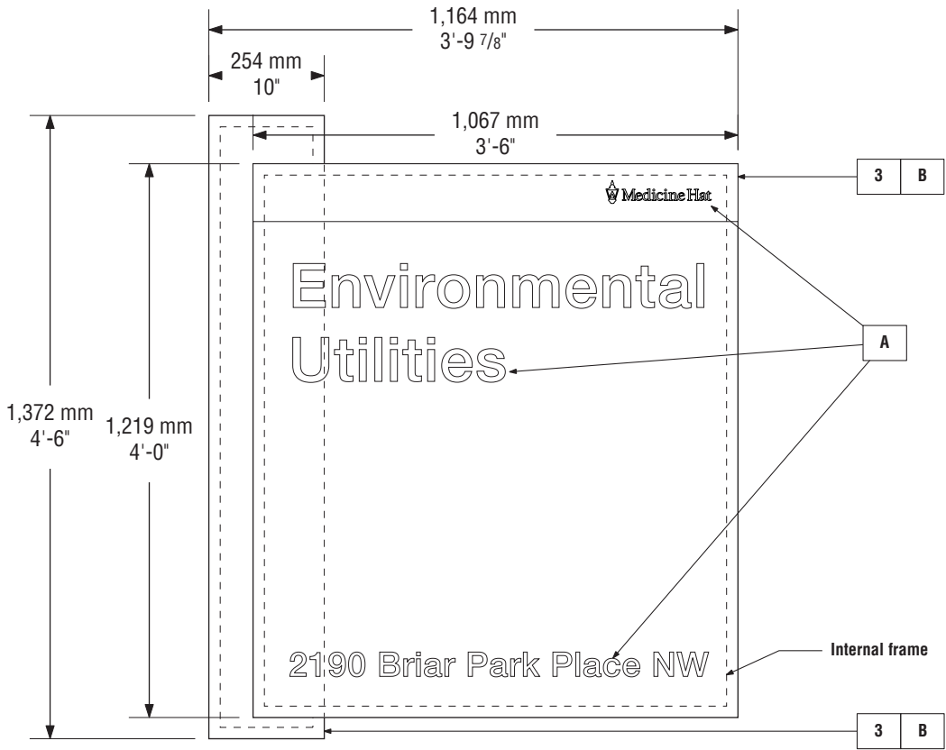
IDF-3 Wall Mounted Facility ID • Front View (Typical)
