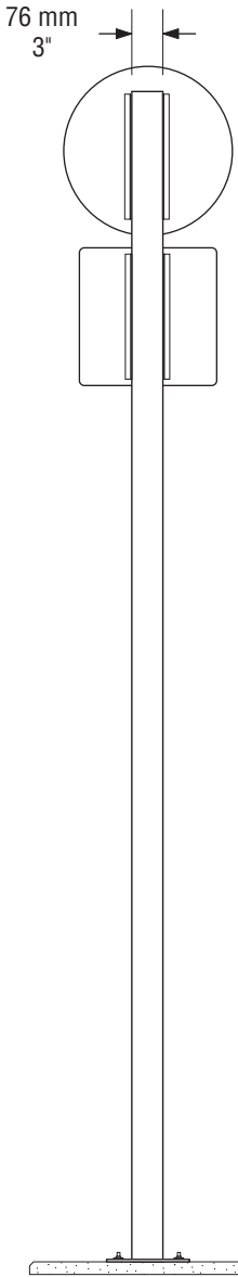
D-2 Trail Connect • Rear View (Typical)
