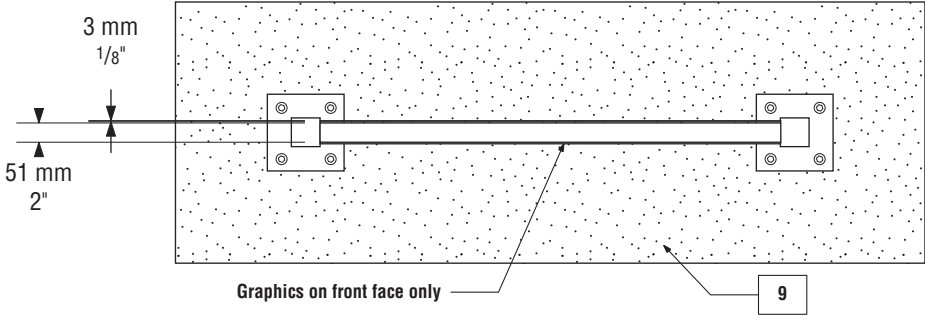
IN-3 Tertiary Information Hub • Top View (Typical)
