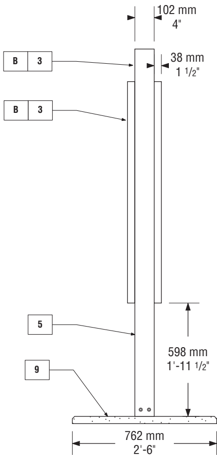
IDF-1 Freestanding Facility Identification • Side View (Typical)
