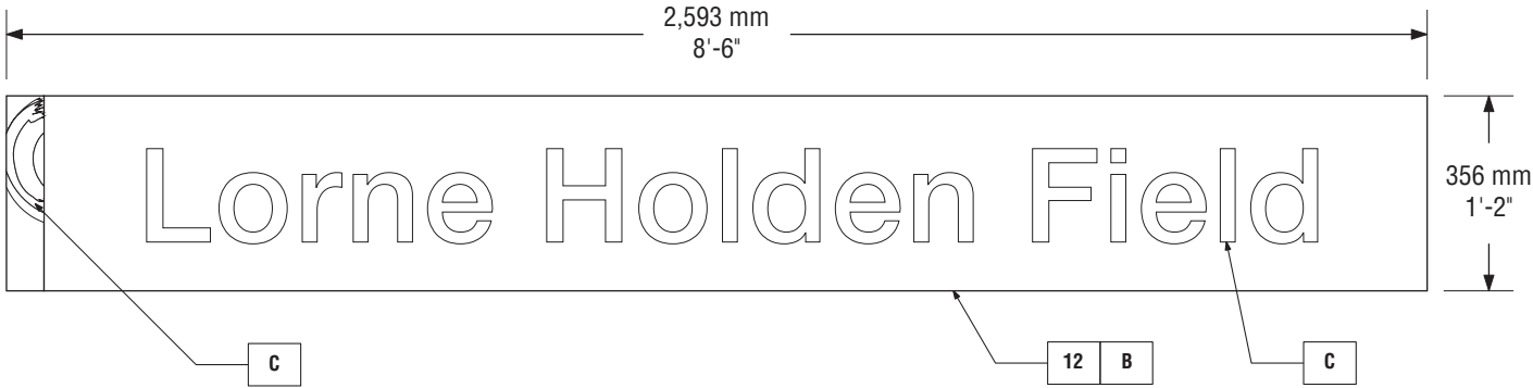
IDP-7 Field Identification • Front View (Typical)
