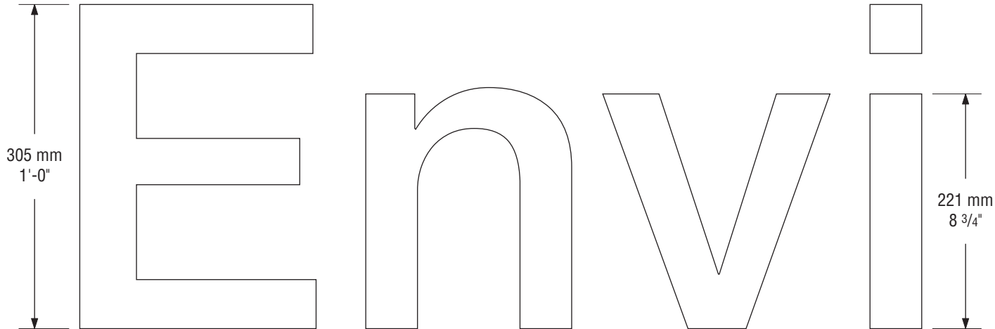
ID-4 Wall Mounted Dimensional Letters • Front View (Detail)
