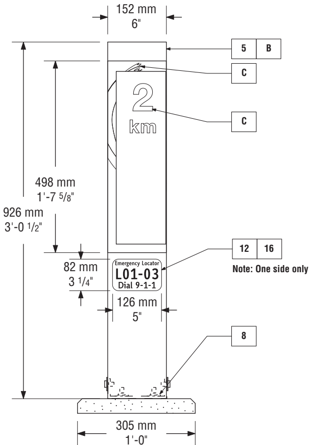
D-3 Distance Marker • Side A (Typical)
