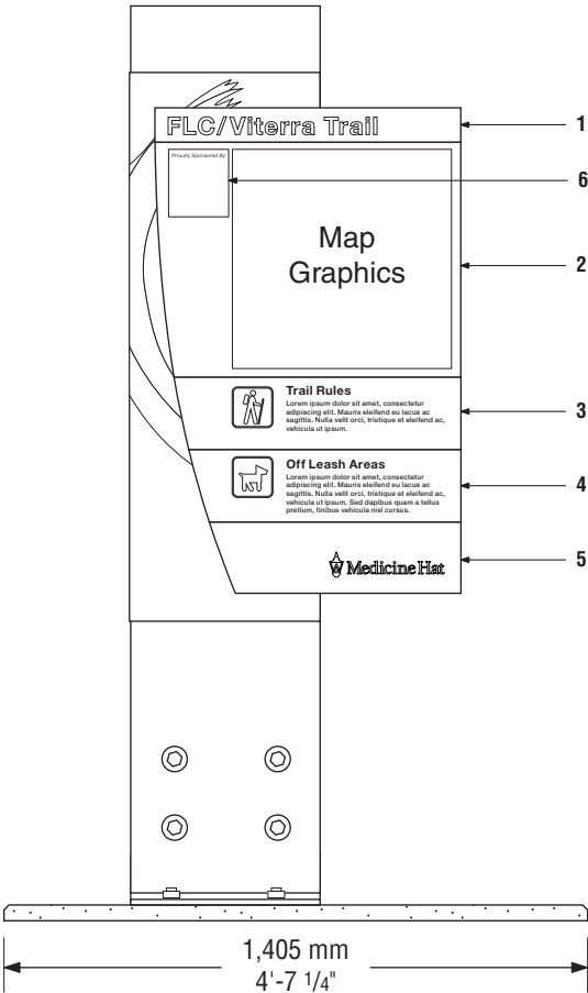
IN-2 Secondary Information Hub • Panel Dimensions (Typical)
