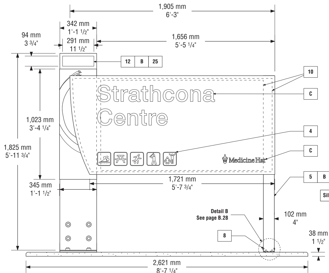
IDP-3 Tertiary Park Identification • Front View (Typical)
