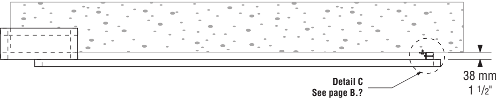
IDF-2 Retrofit Facility ID • Top View (Typical)
