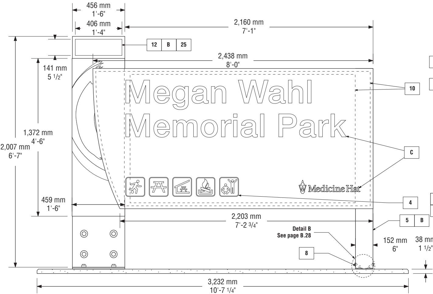
IDP-2 Secondary Park Identification • Front View (Typical)
